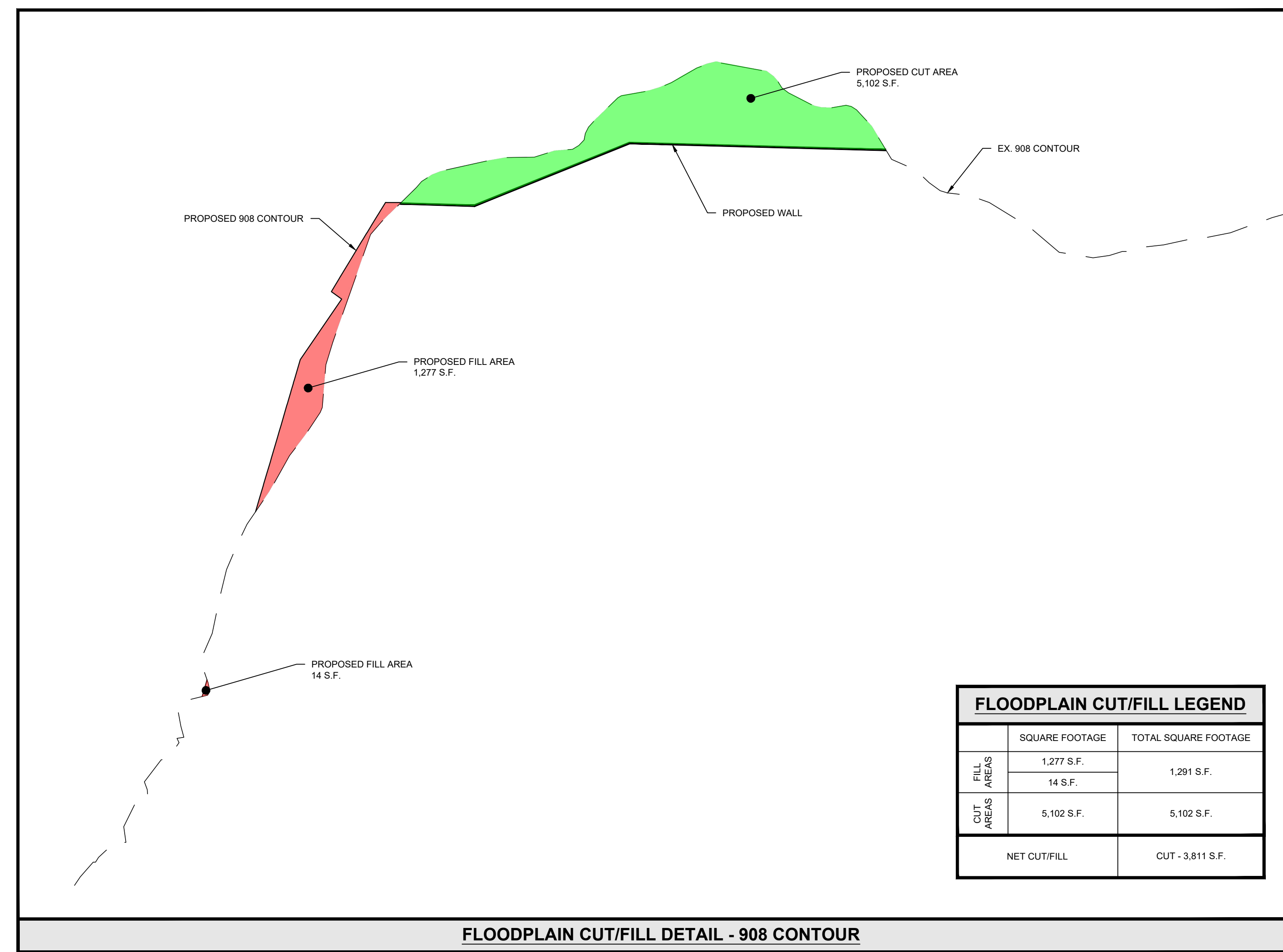
FLOODPLAIN CUT/FILL DETAIL - 908 CONTOUR
