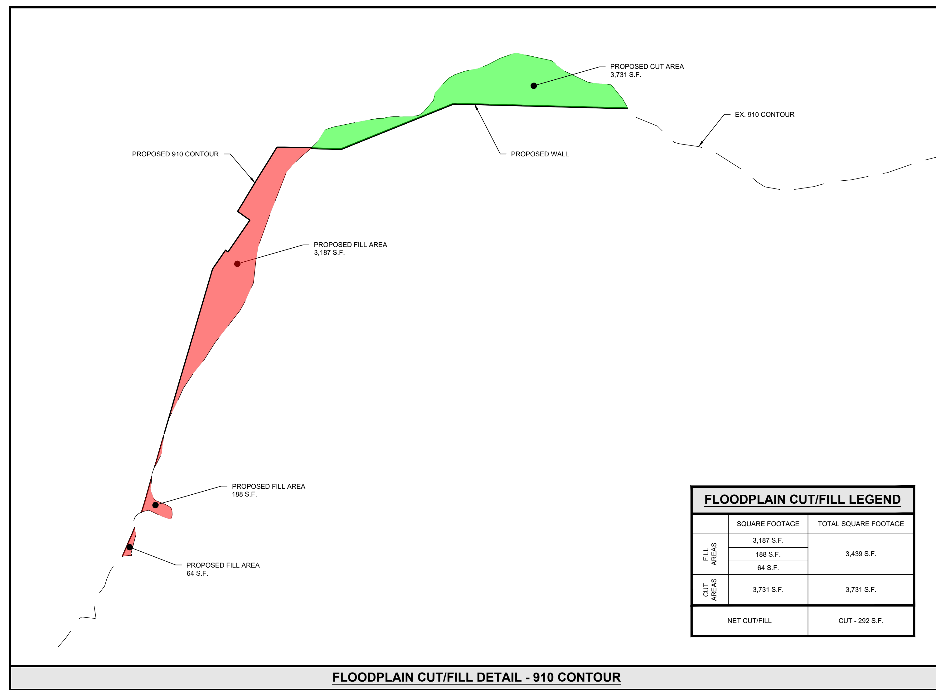
FLOODPLAIN CUT/FILL DETAIL - 910 CONTOUR
