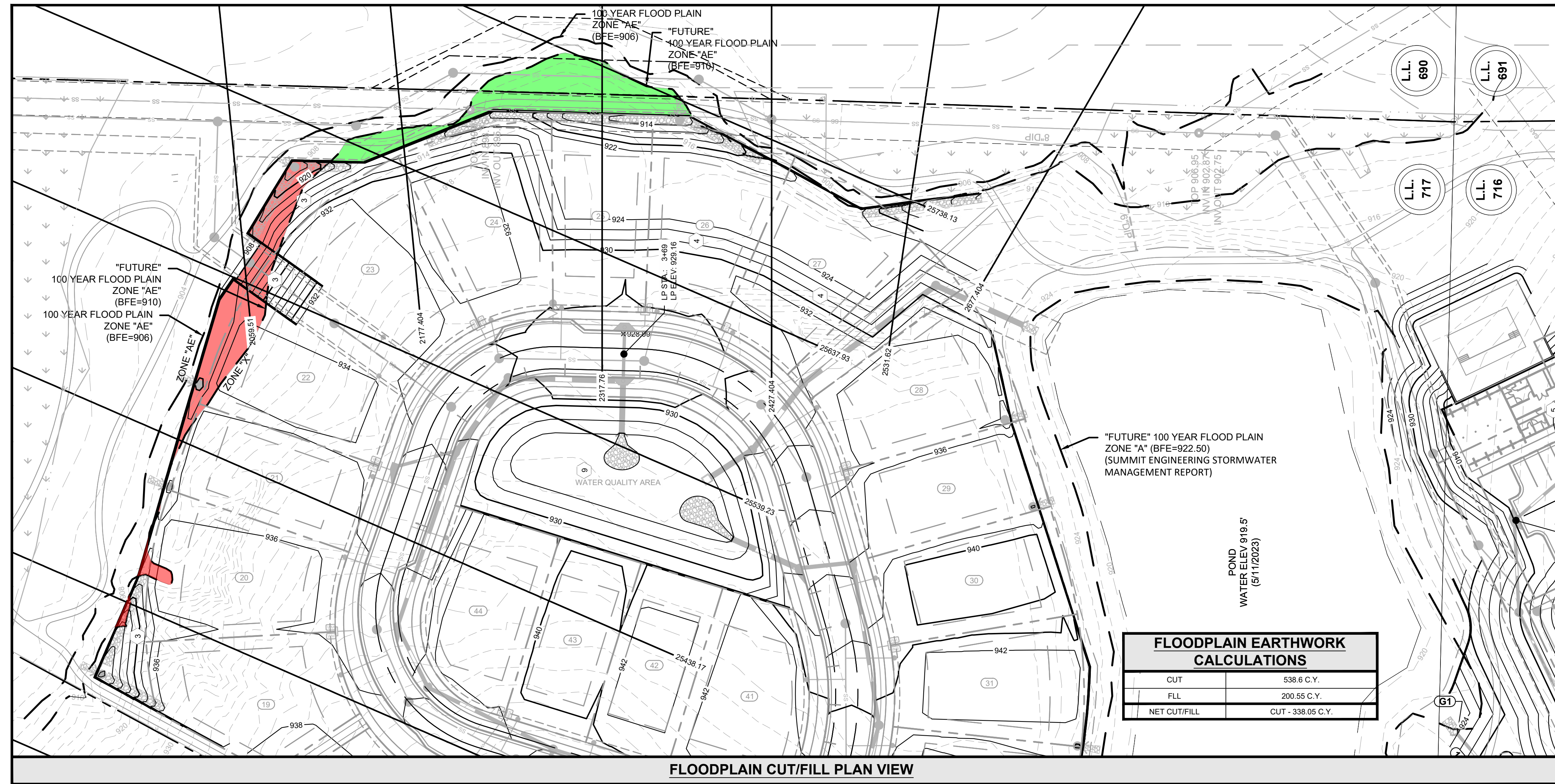
FLOODPLAIN CUT/FILL PLAN VIEW
