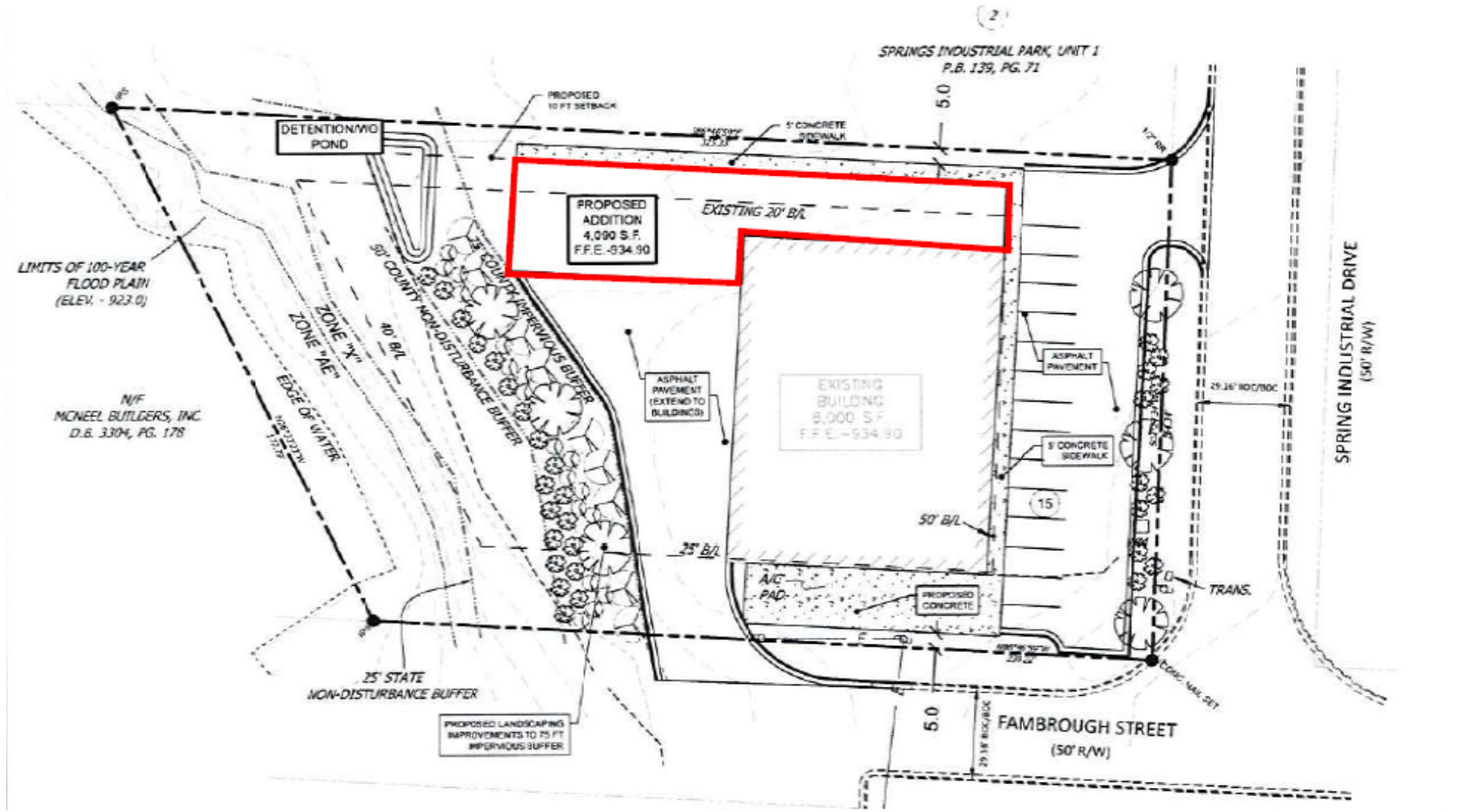
Figure 2. Proposed building 4090-sf addition outlined in red.
