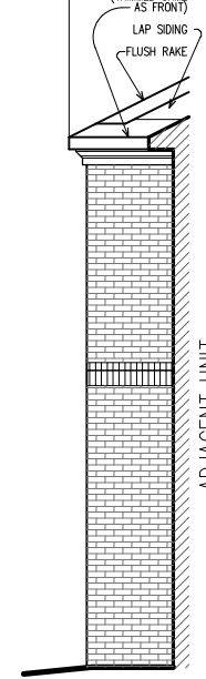
Front Elevation, Lots - 56,58 Right and Left Side Returns
