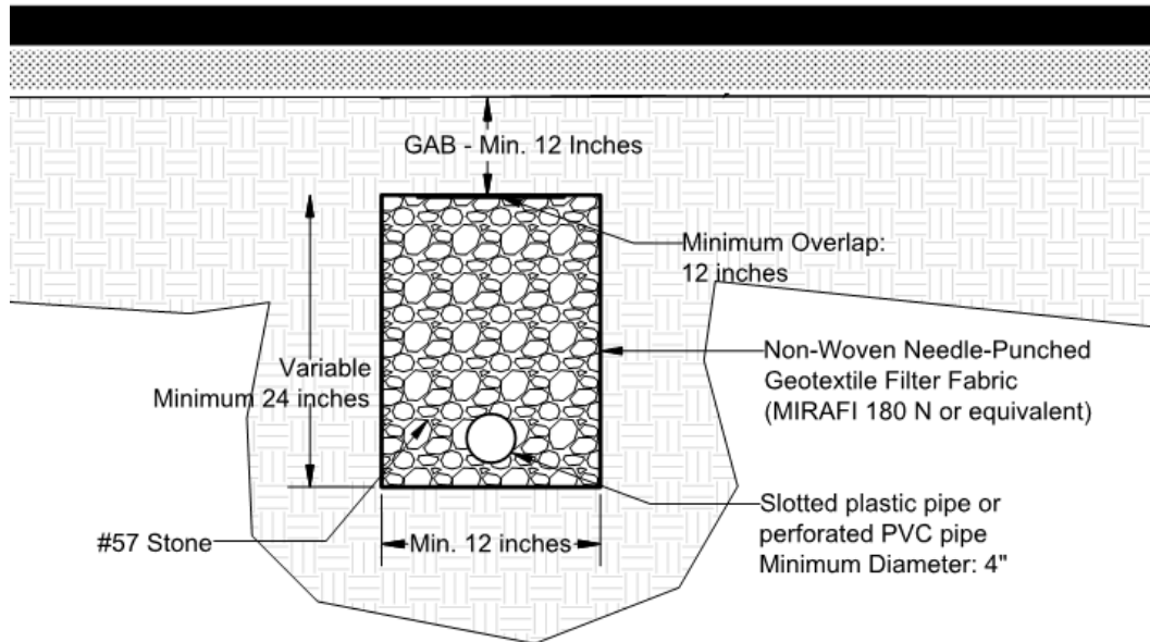
Typical Trench Drain Detail
